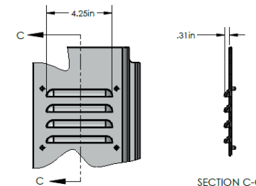
VENTING
